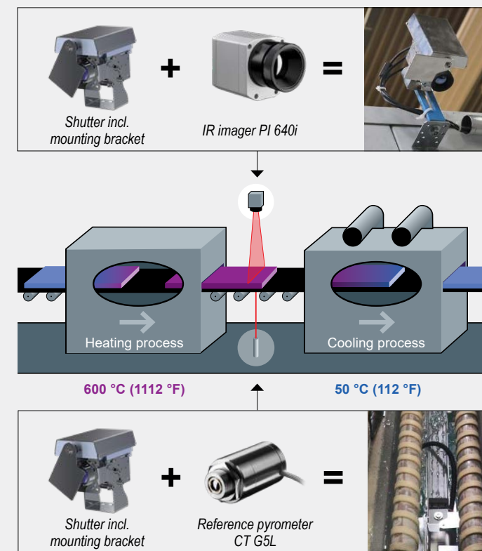
Positioning of IR camera and reference pyrometer in a Top-Down Glass Inspection System.
